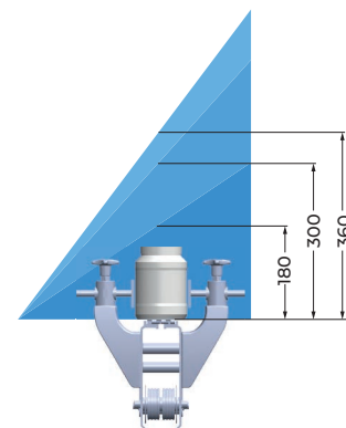
Beam geometry
