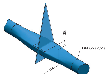
Beam geometry
